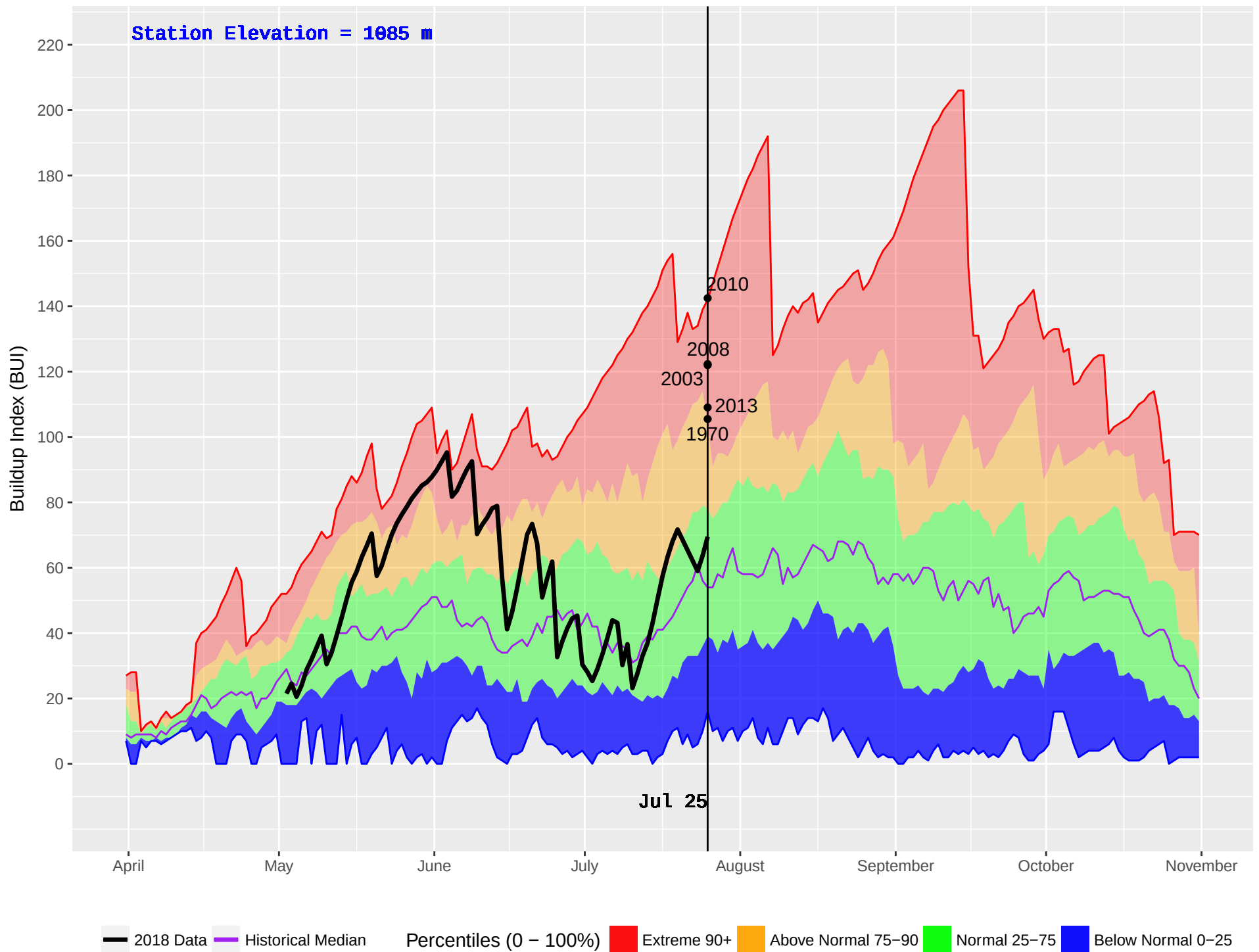
TAUTRI (206) : Historical (1970–2016) and Current (2018) Noon Buildup Index (BUI)
