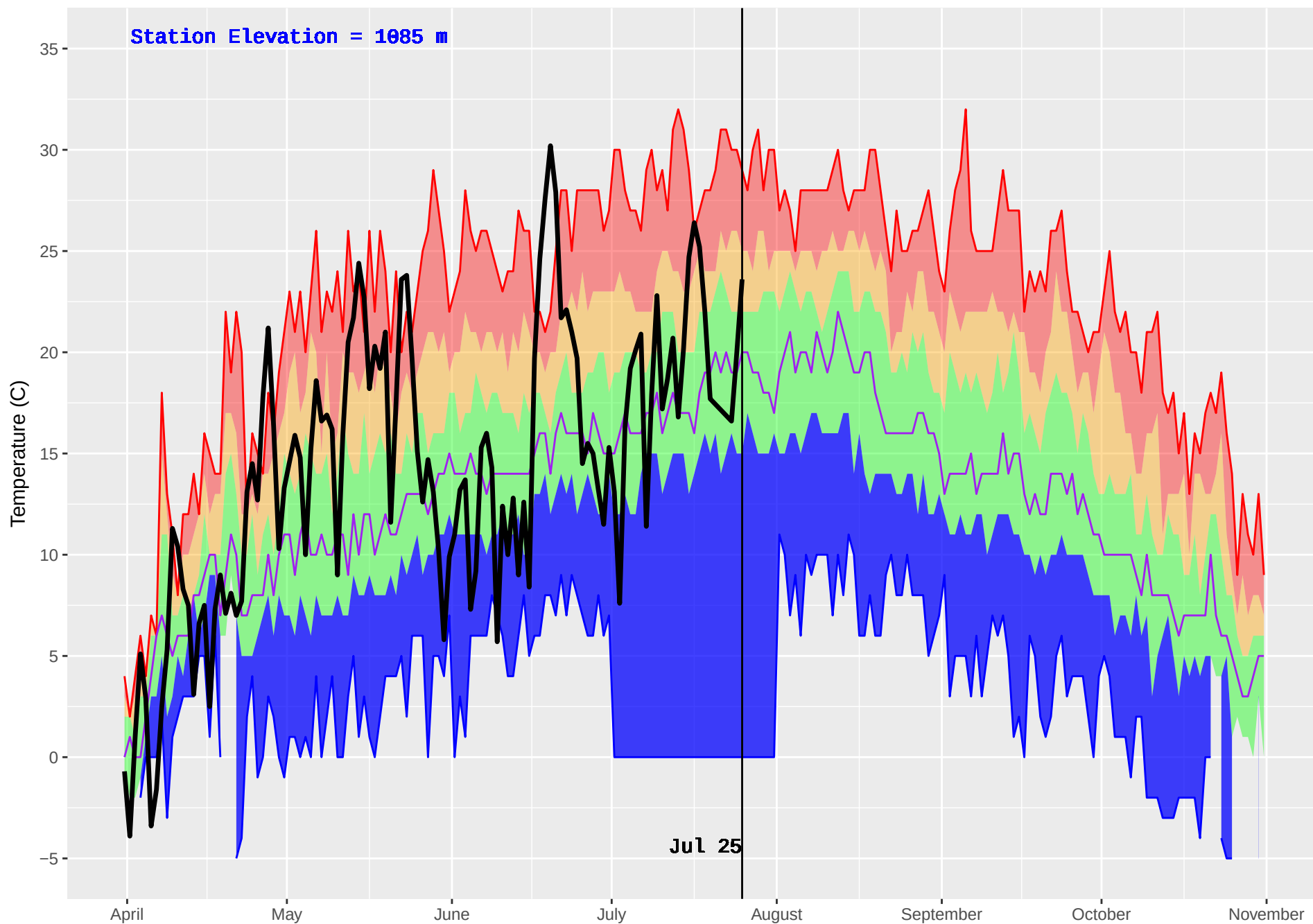
TAUTRI (206) : Historical (1970–2016) and Current (2018) Noon Temperature
