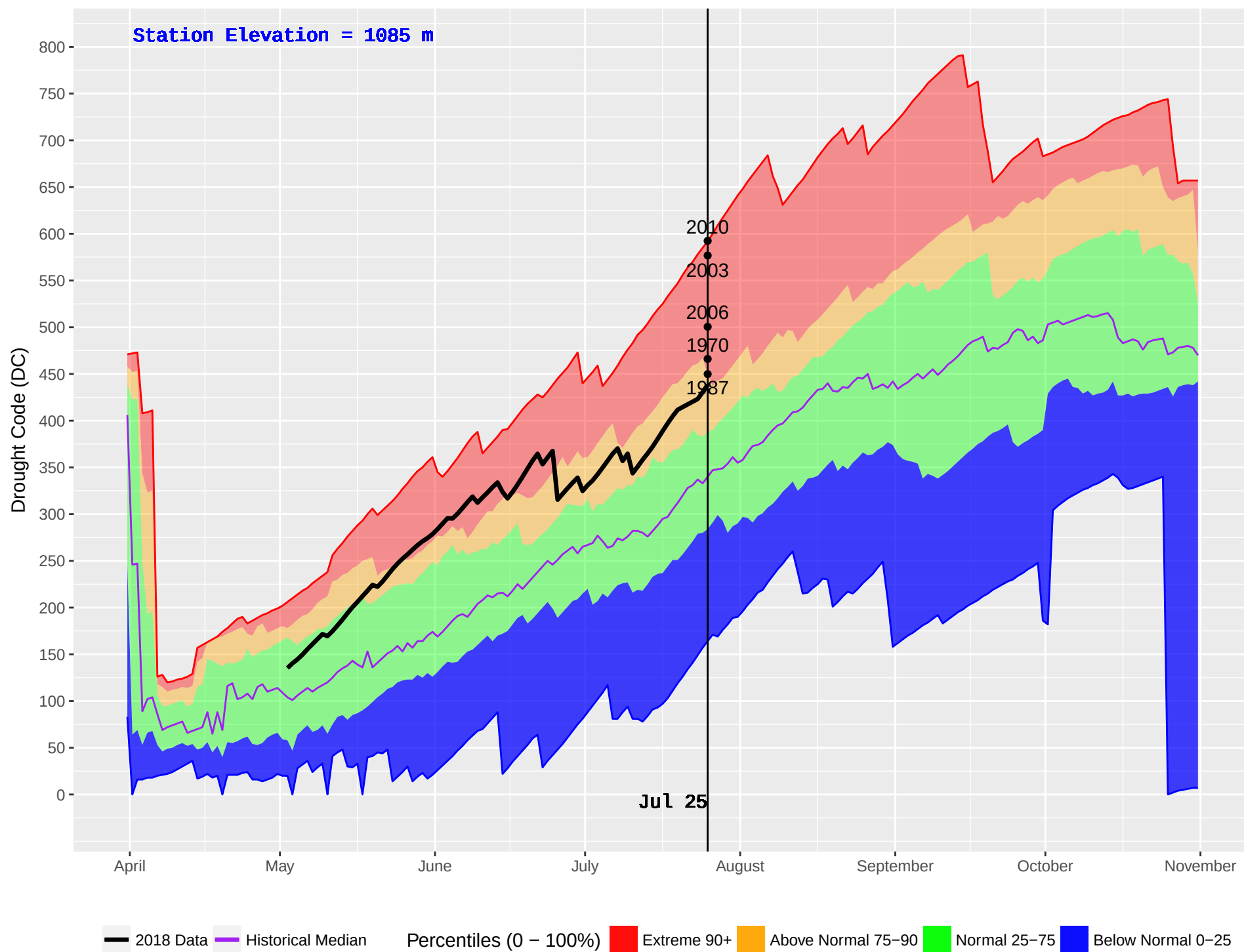
TAUTRI (206) : Historical (1970–2016) and Current (2018) Noon Drought Code (DC)
