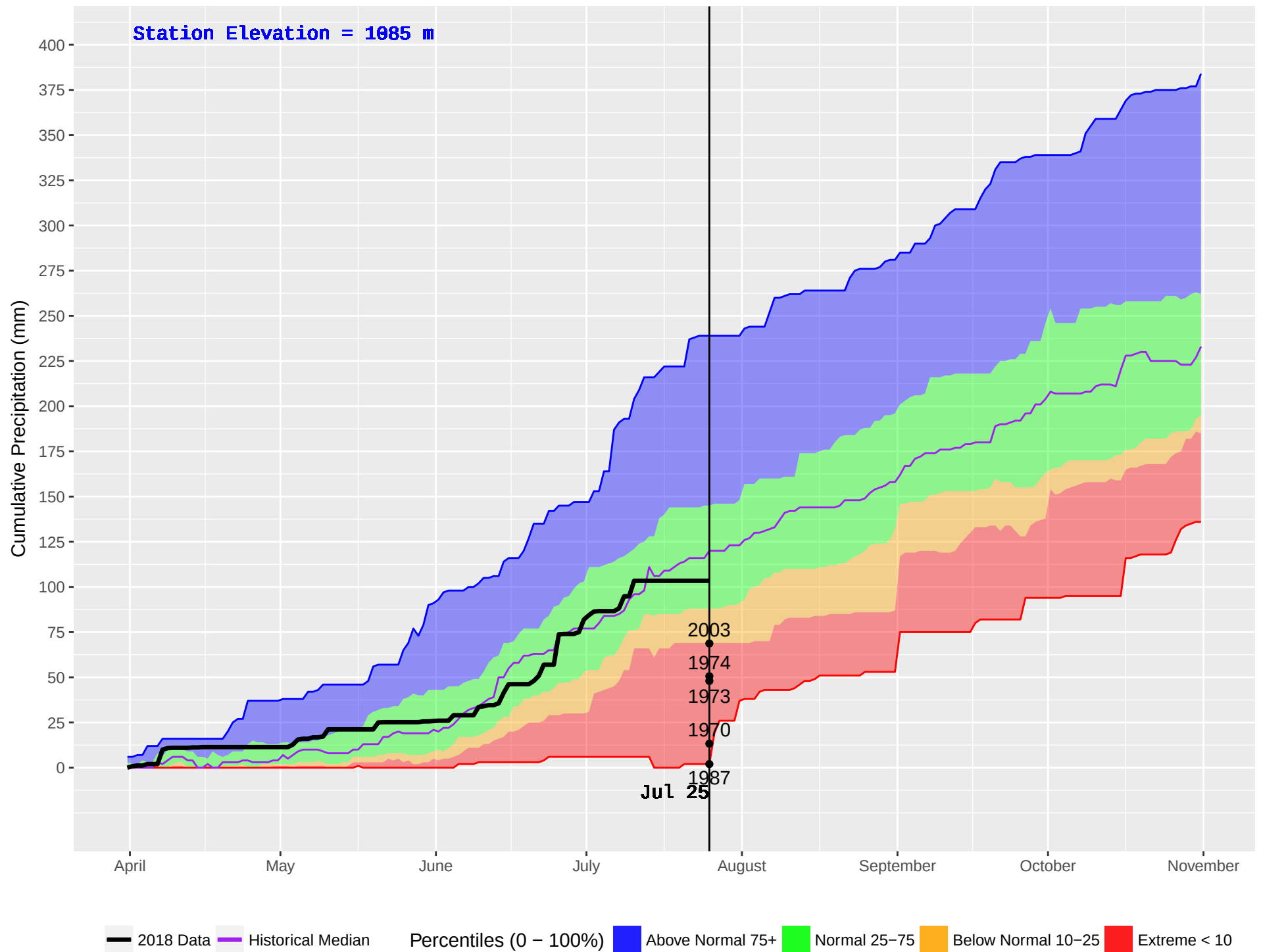
TAUTRI (206) : Historical (1970–2016) and Current (2018) Noon Cumulative Precipitation
