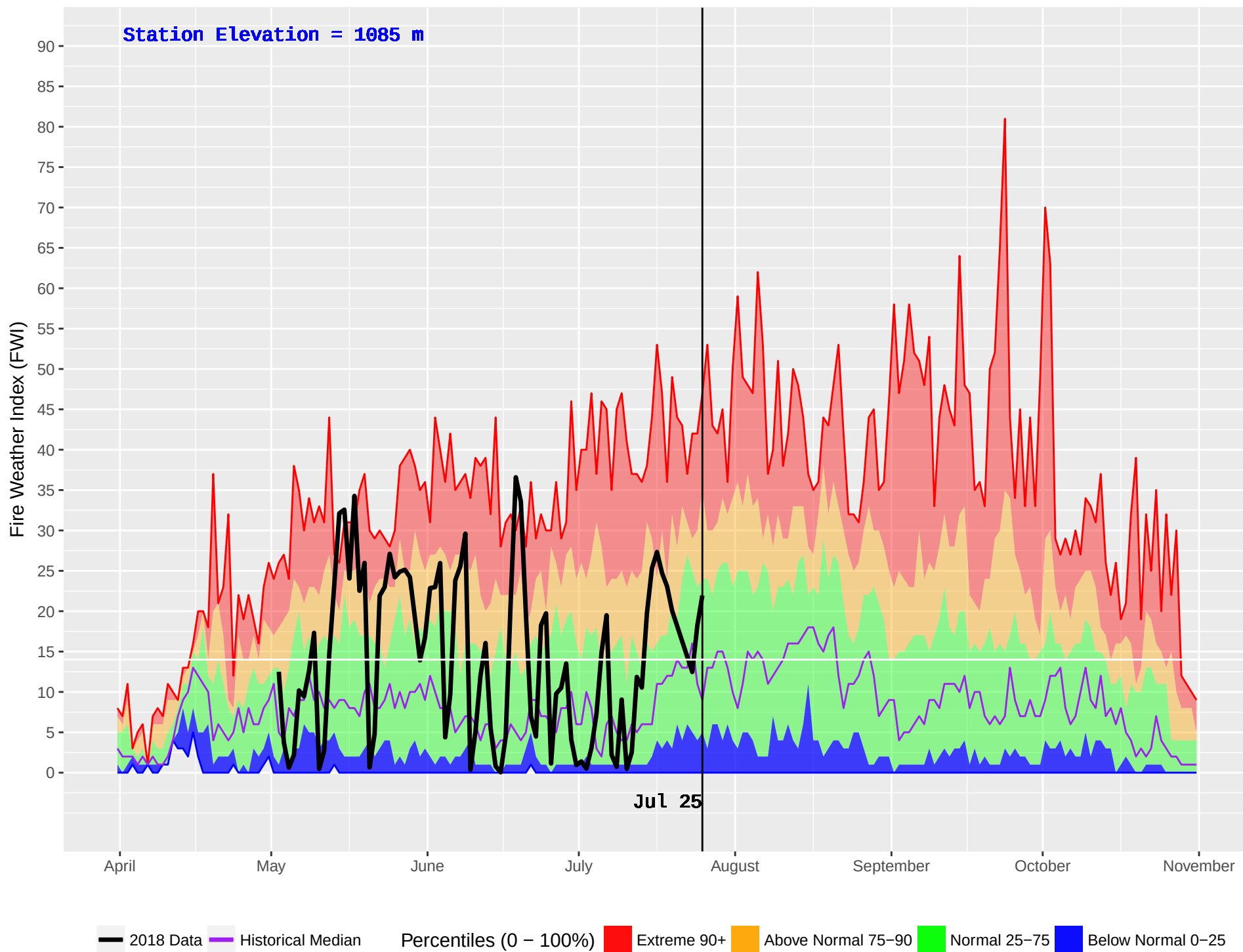
TAUTRI (206) : Historical (1970–2016) and Current (2018) Noon Fire Weather Index (FWI)
