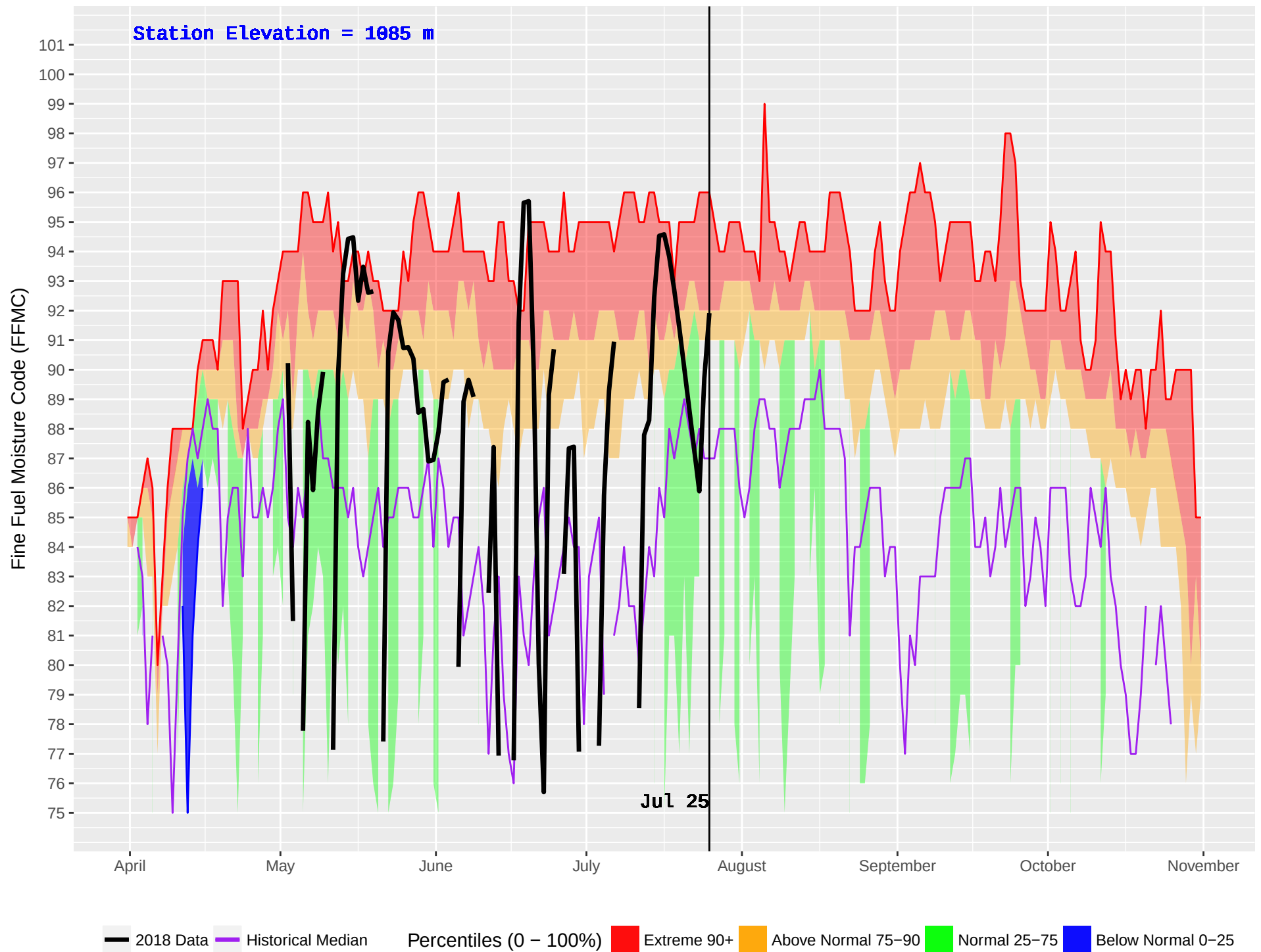
TAUTRI (206) : Historical (1970–2016) and Current (2018) Noon Fine Fuel Moisture Code (FFMC)
