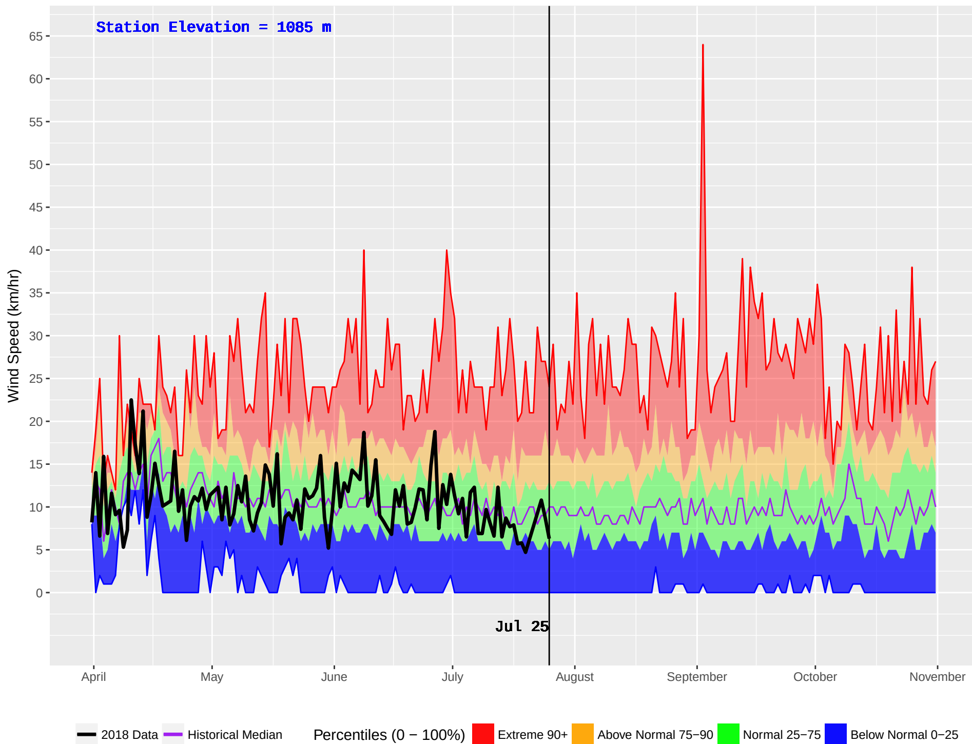
TAUTRI (206) : Historical (1970–2016) and Current (2018) Noon Wind Speed
