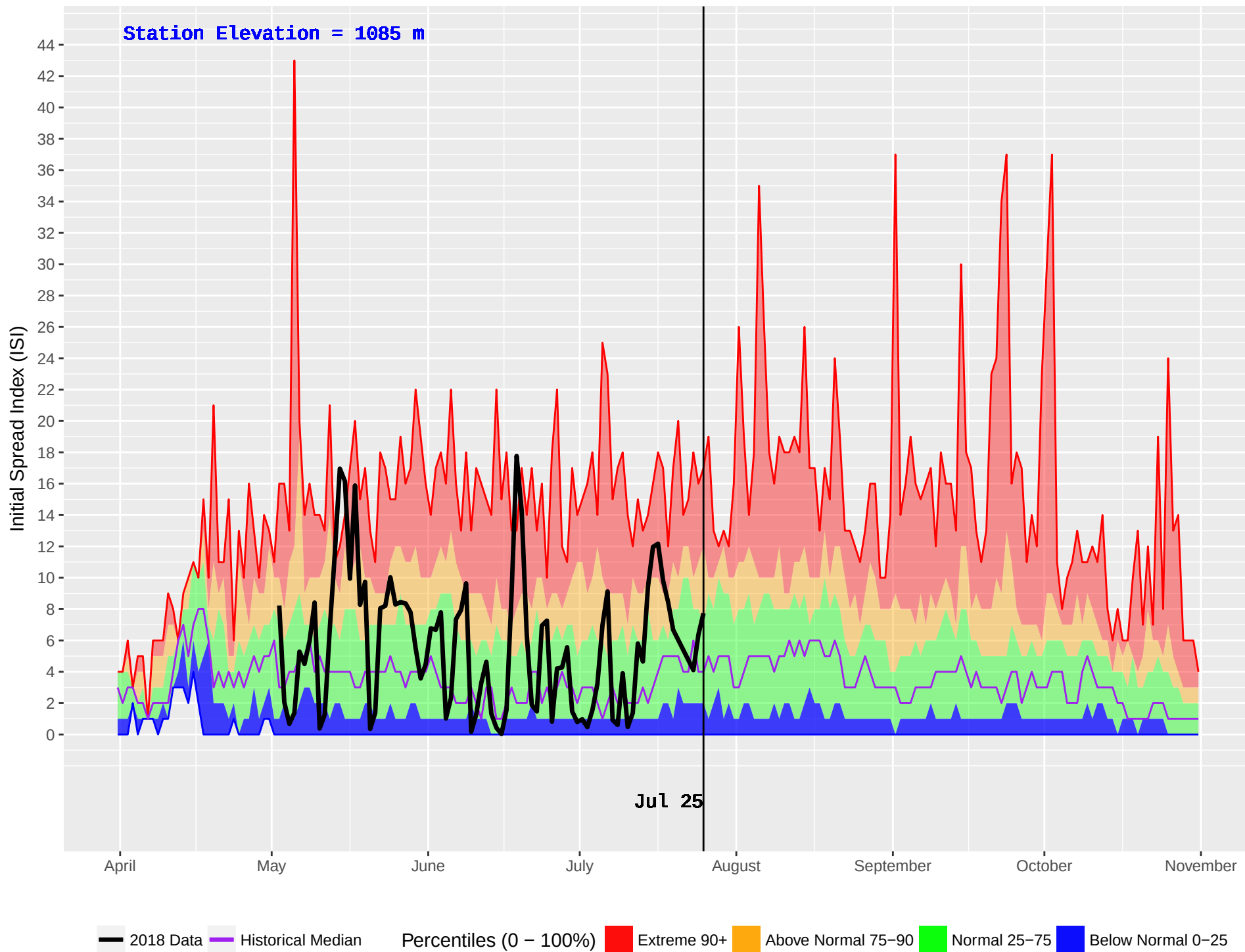
TAUTRI (206) : Historical (1970–2016) and Current (2018) Noon Initial Spread Index (ISI)
