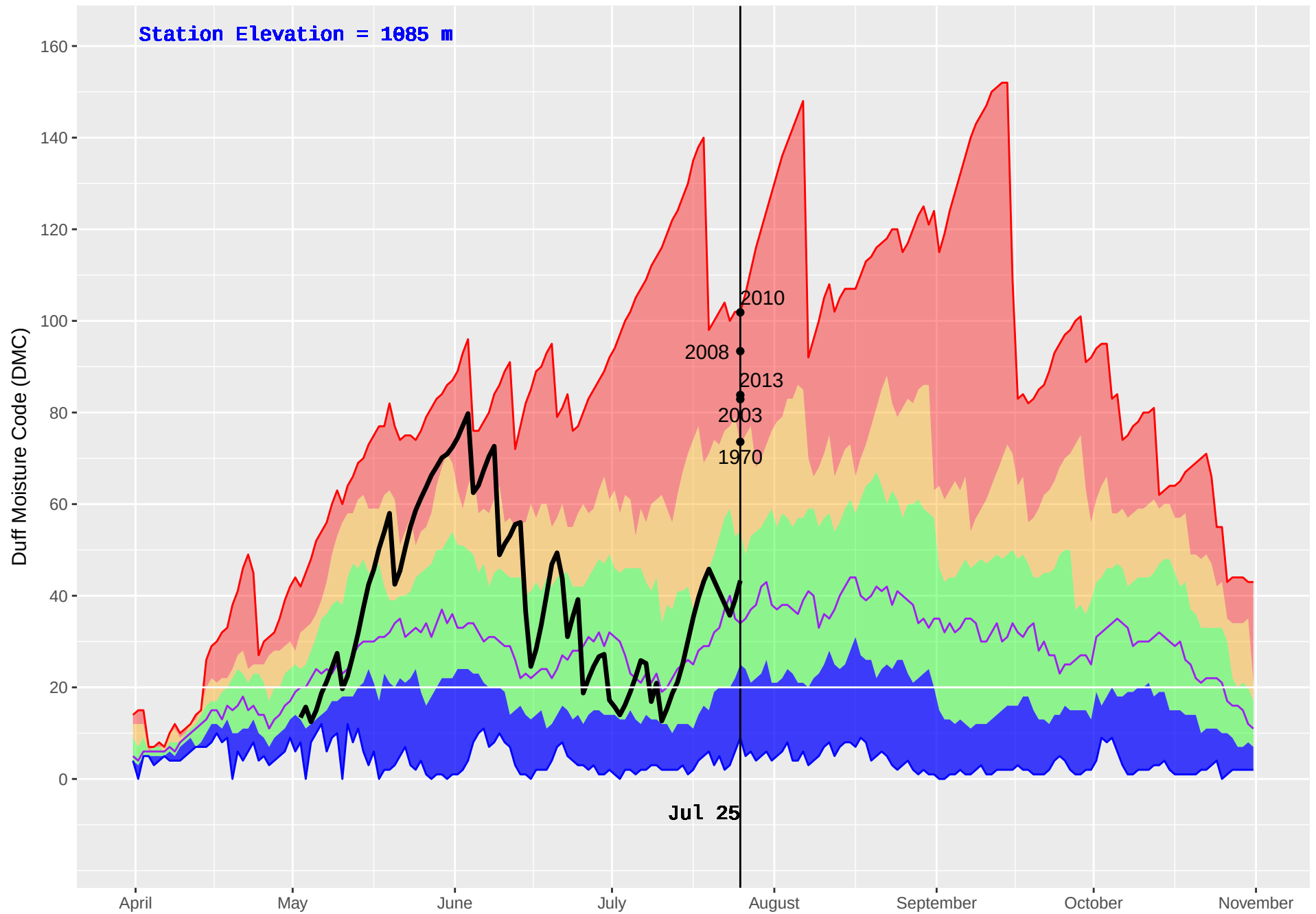
TAUTRI (206) : Historical (1970–2016) and Current (2018) Noon Duff Moisture Code (DMC)
